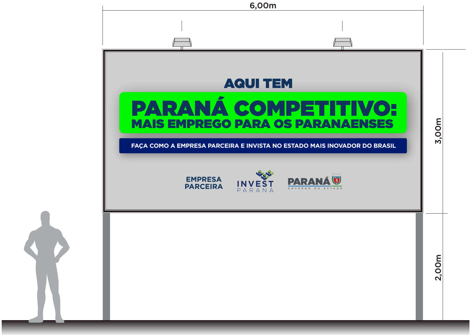
Vista frontal
